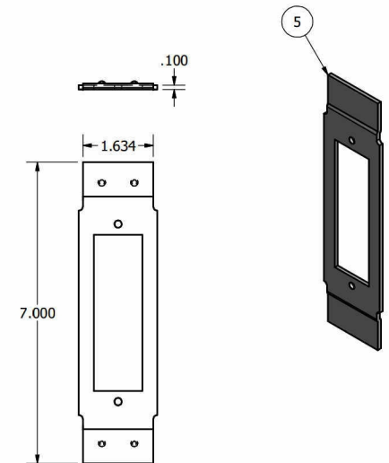
Door Strike Reinforcement (12ga Galvaneal)
